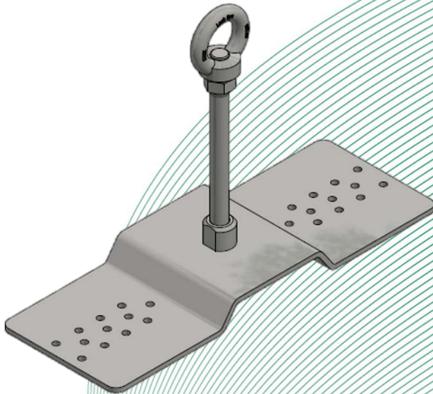
Fig. 1: Anchor device, type: ABS-Lock® X-SW-6
