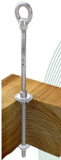
Fig. 1: Anchor device, type: ABS-Lock® III
